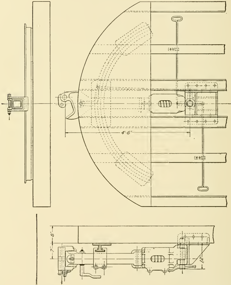
Fig. 118. Plan and Elevation of Standard M. C. B. Coupler
